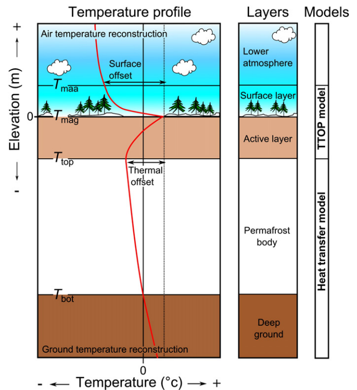
Fig. 4. Permafrost model showing five distinct layers and the temperature vertical profile curve (red line) (modified from Riseborough et al., 2008). T_{\text{bot}} : mean annual temperature at the bottom of the permafrost. T_{\text{top}} : mean annual temperature at the top of the permafrost. T_{\text{maa}} : mean annual air temperature. T_{\text{mag}} : mean annual ground surface temperature.
