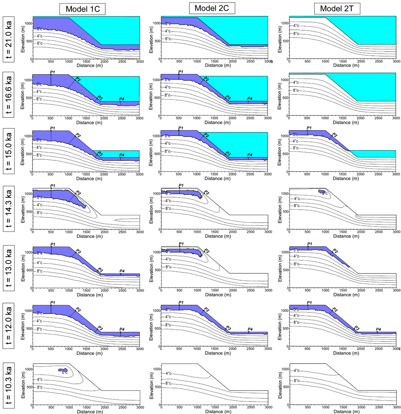
Fig. 9. 2D temperature distributions simulated for the three models 1C, 2C and 2T (1: constant n -factors; 2: variable n -factors; C: cold glacier; T: temperate glacier) at different times, applying the temperature curves in Fig. 5. The permafrost and glacier extensions are shown with deep and light blue colors, respectively. P1 to P4 show the locations where permafrost thickness values were extracted (Table 3).
