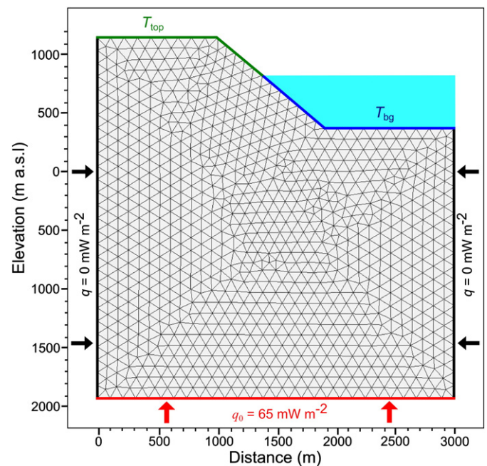
Fig. 7. 2D Séchilienne slope model with the applied boundary conditions. The glacier at 15.6 ka is in blue. T_{\text{top}} : Temperature deduced from the TTOP model and imposed at the surface. T_{\text{bg}} : Temperature at the base of the glacier. The thickness of the glacier varies between 0 and 820 m.
